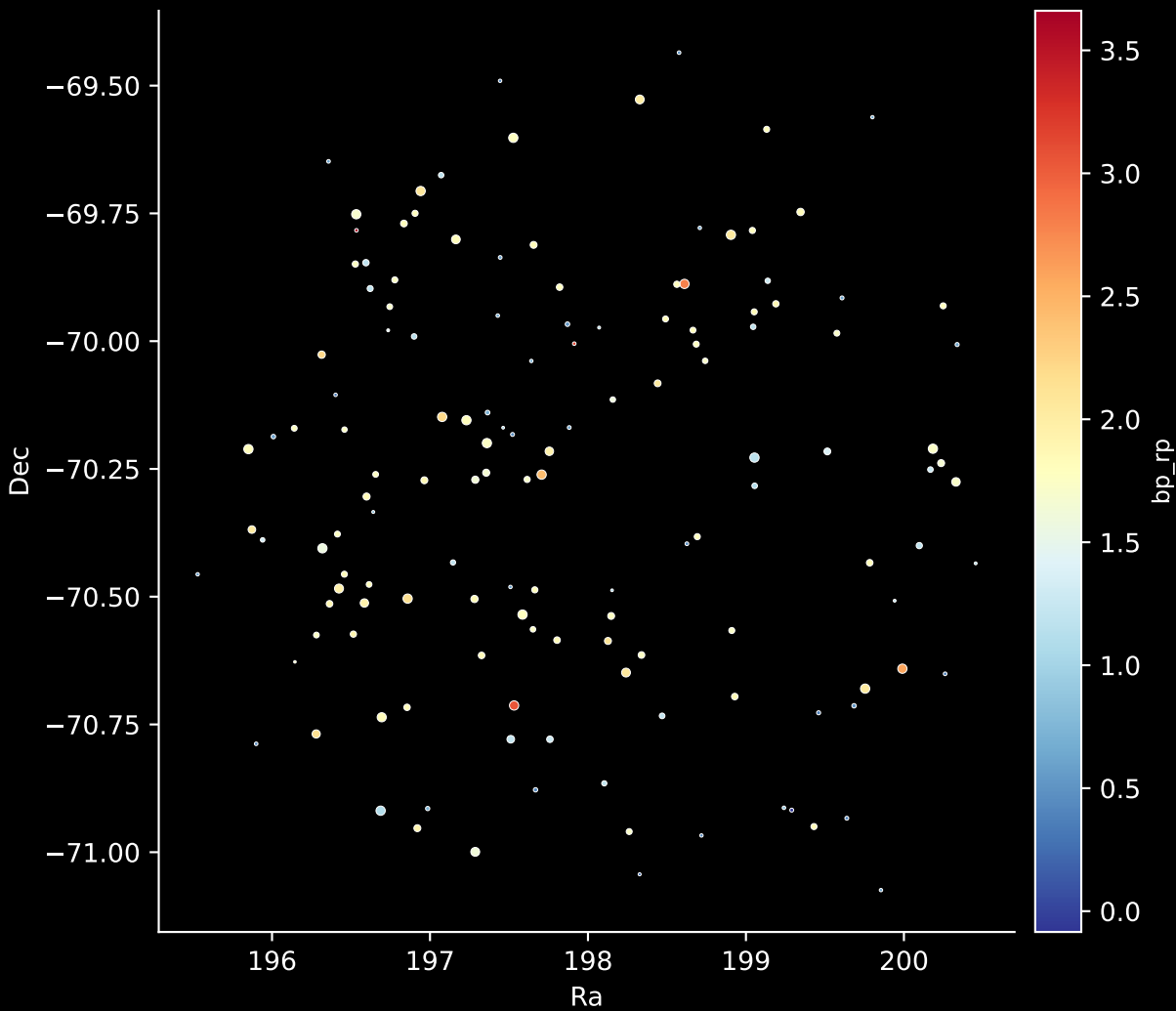
APOGEE DR17 Field: [LMC17] Stars: 140
