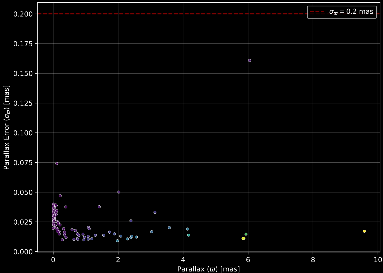
APOGEE DR17 Field: [LMC17] Parallax Quality (n= 140)
