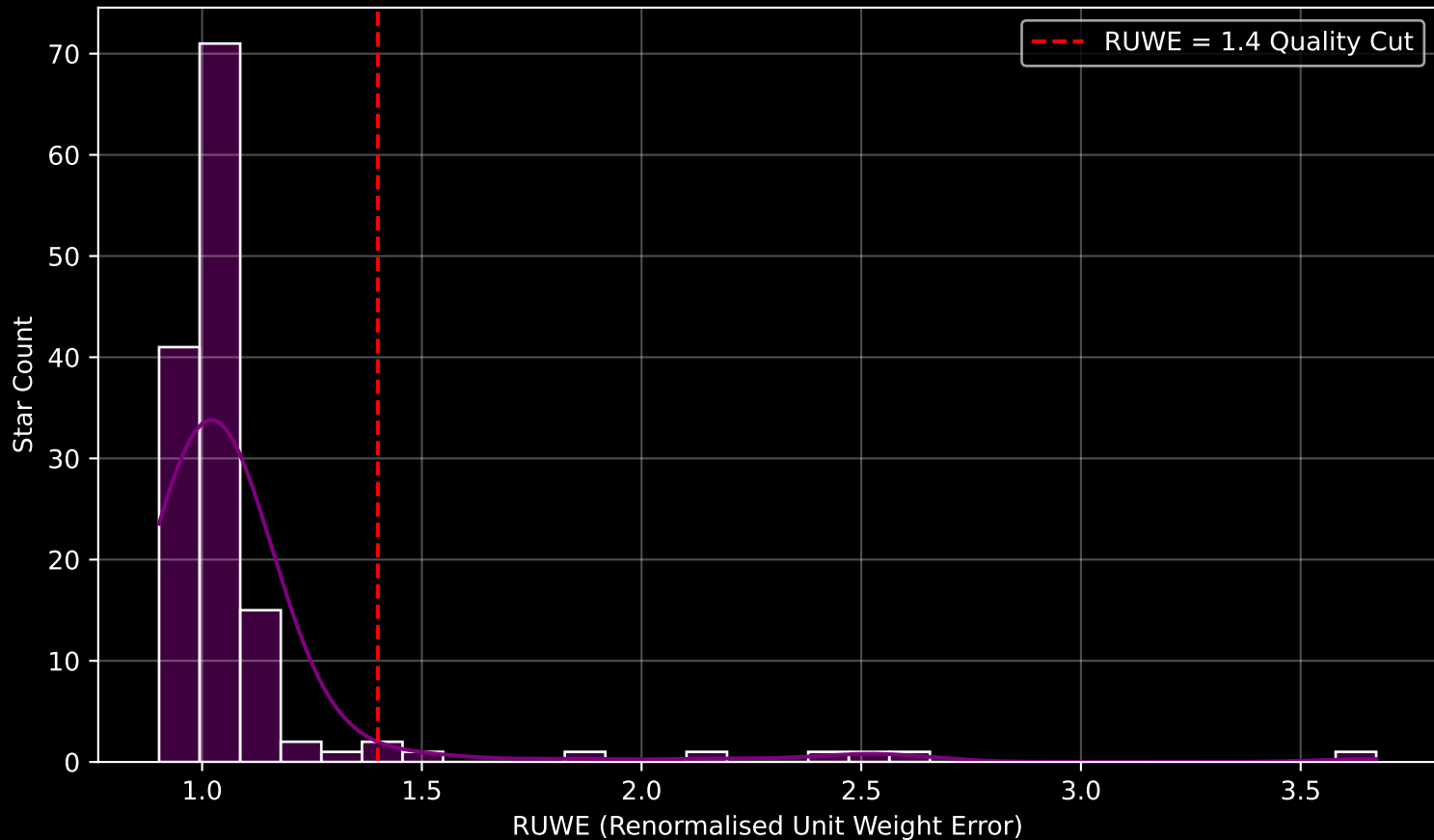
GAPOGEE DR17 Field [LMC17] RUWE Distribution (n= 139)
