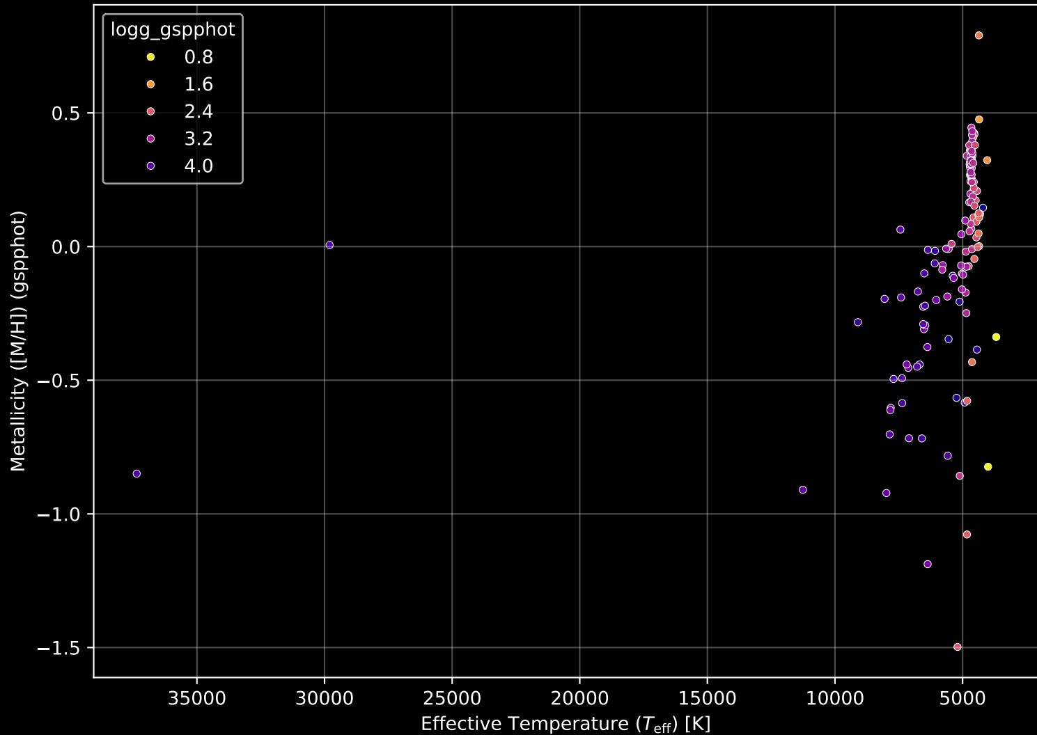
APOGEE DR17 Field: [LMC17] Stellar Population Parameters (n= 140)
