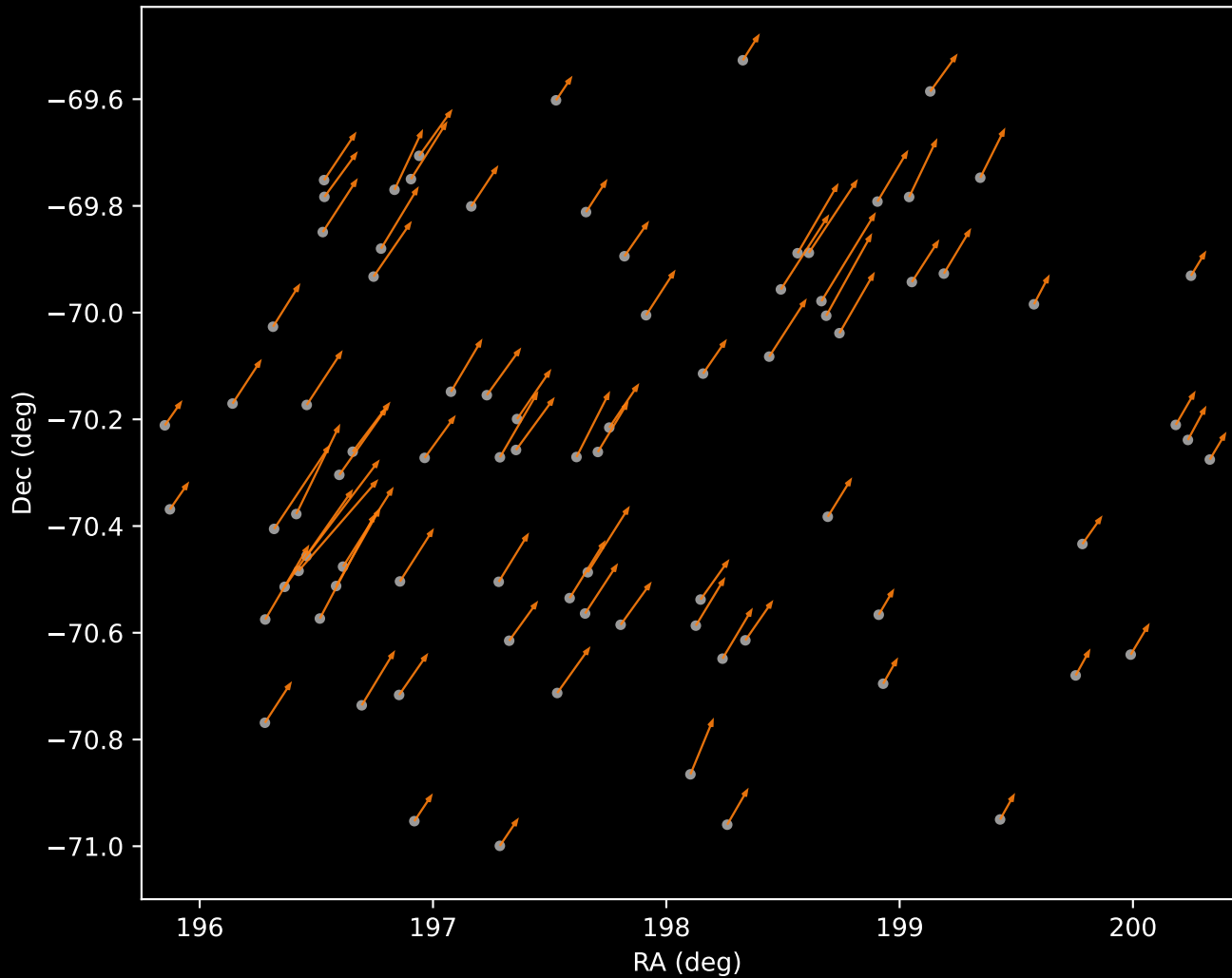
APOGEE DR17 Cluster 2 Proper Motion Vectors (n=84)
