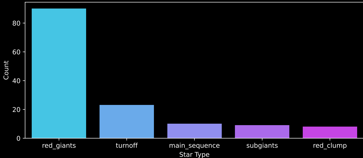
APOGEE DR17 Field: [LMC17] Count plot of Star Type
