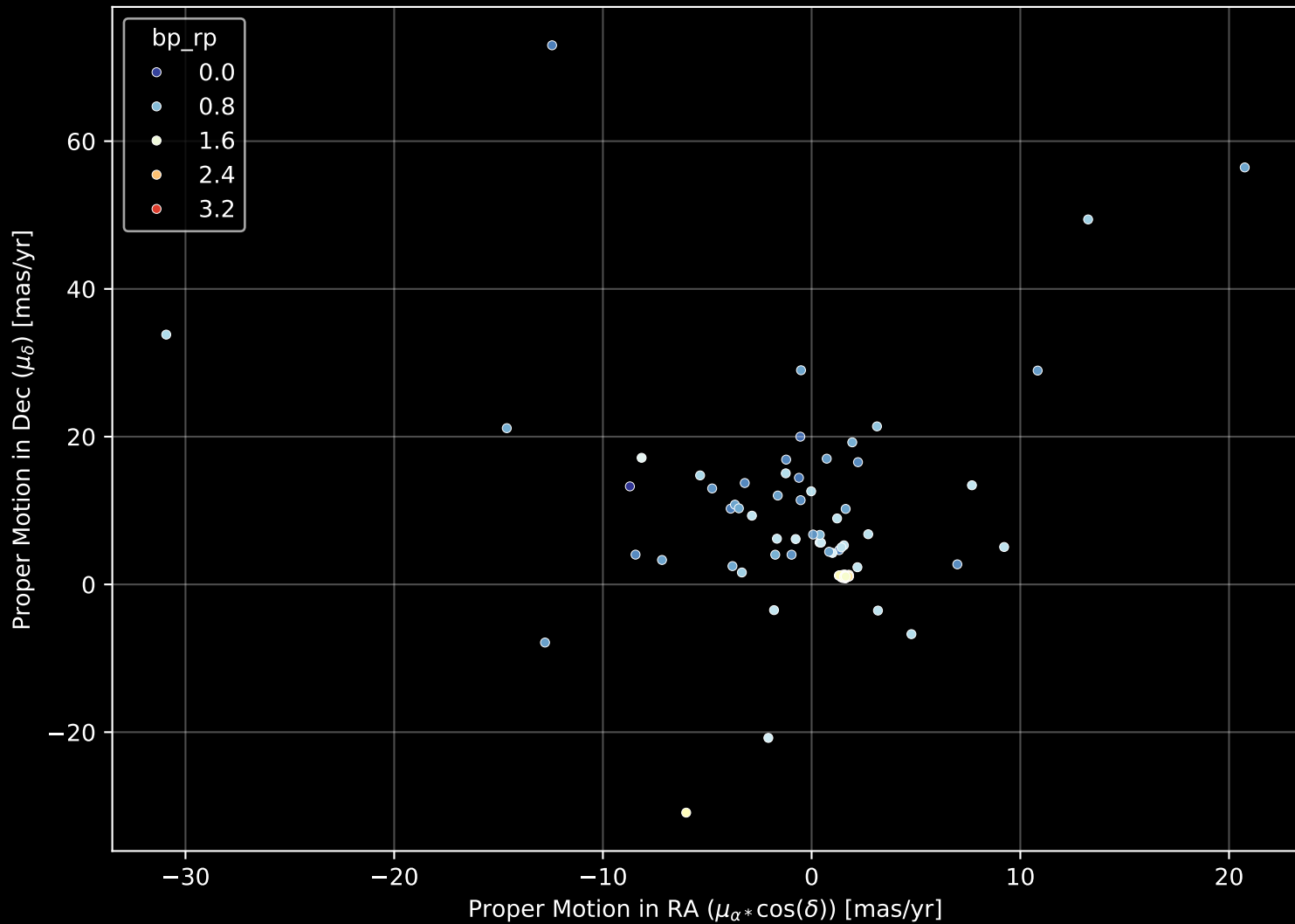
APOGEE DR17 Field: [LMC17] Proper Motion Diagram (n= 140)
