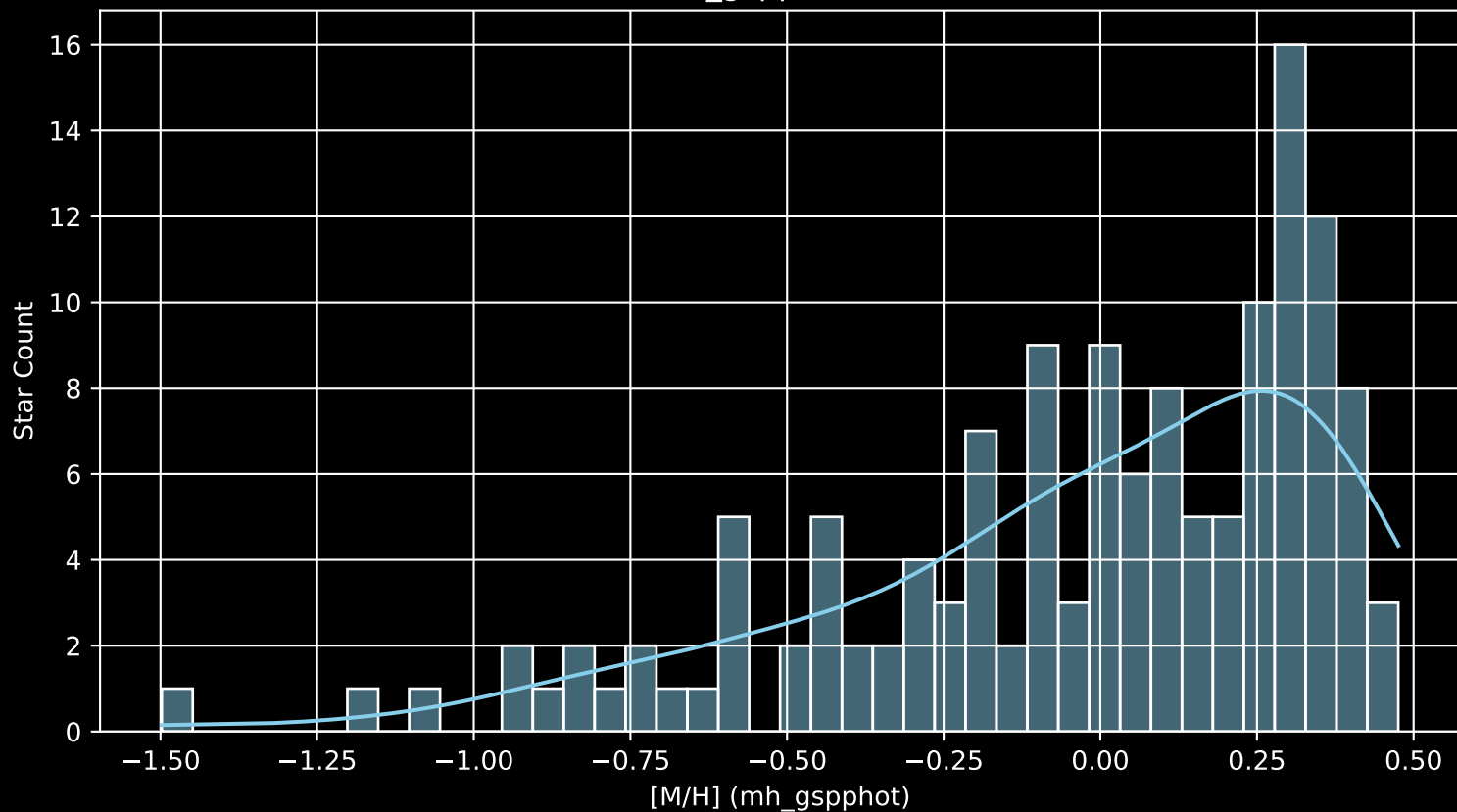
APOGEE DR17 Field: [LMC17 [M/H] (mh_gspphot) (n= 139)
